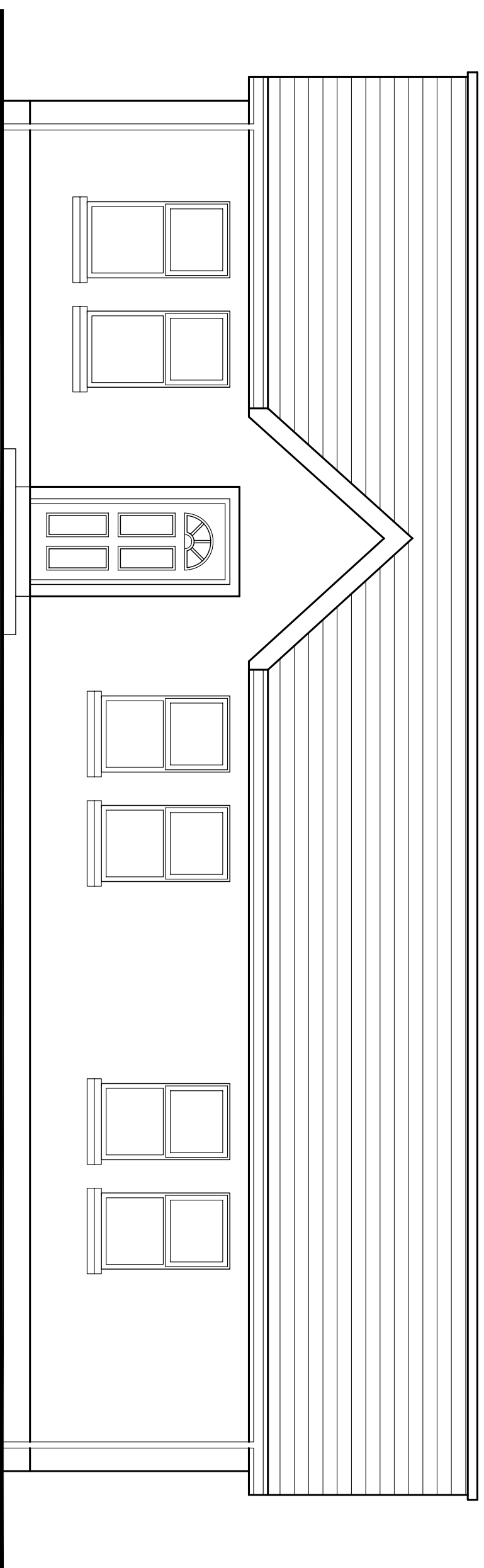
front elevation
